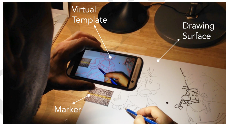
Fig. 2. ML virtual tracing method. The mobile phone renders a virtual template image ( red contour line) and a live video stream of the drawing surface (a hand and a paper) onto device screen allowing the user to follow the red line. The marker is required for camera pose. Every time the marker is moved (e.g. because it falls out of camera's field of view or is in the way of pencil), the user needs to align the virtual template (red line) with what has been drawn thus far using touchscreen gestures.
